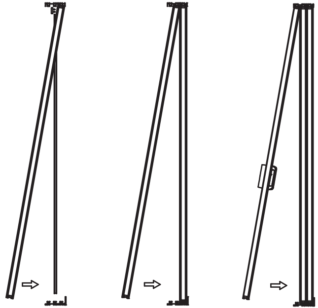
Panel Installation (2 and 4 Panel Doors Similar)
