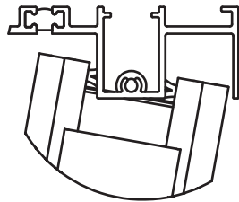
Panel Installation (2 and 4 Panel Doors Similar)
