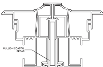
Series 150 Mullion Assembly:
