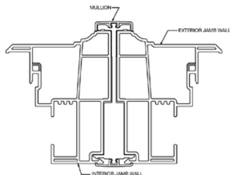
Series 160 Mullion Assembly:
